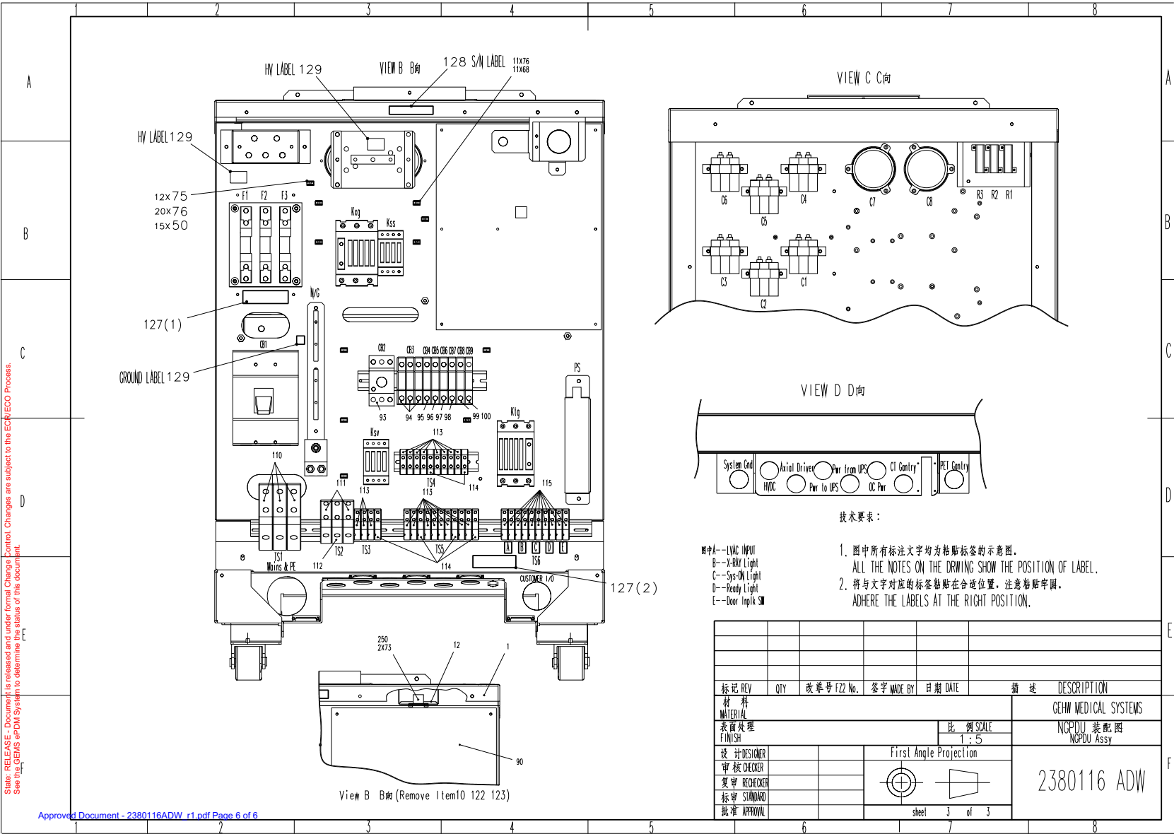
Figure 3-3 NGPDU ASSEMBLY3 (2380116, sheet 3, rev 1)
