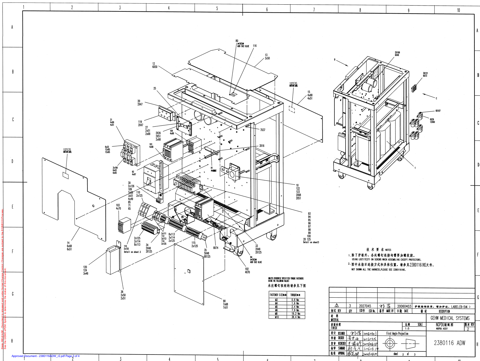
Figure 3-2 NGPDU ASSEMBLY3 (2380116, sheet 2, rev 2)
