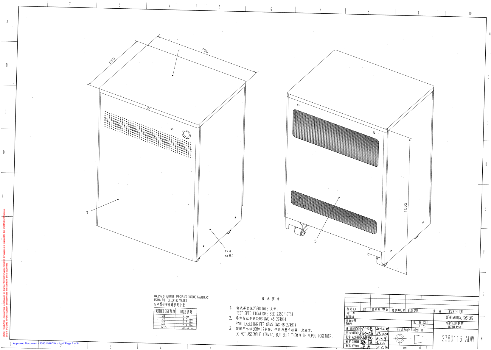
Figure 3-1 NGPDU ASSEMBLY3 (2380116 Sheet 1, rev 1)
